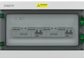
LQX-4/2DC600VL7
