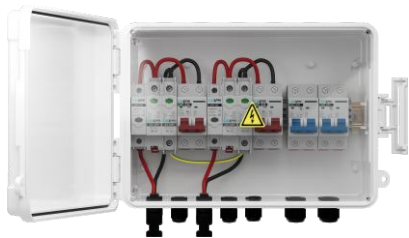
LQX-N2/2DC500VB1-2/2AC220VBB-MP
