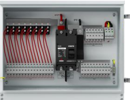
LQT-N/1DC1500VM3
