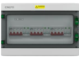
LQX-3/3DC1000VBS
