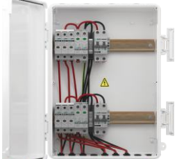
LQX-N6/2DC600VL7
