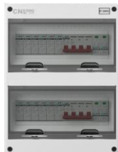
LQX-C6/2DC1000VB1
