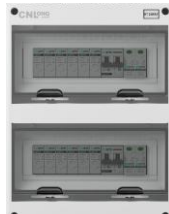
LQX-C6/2DC600VL7
