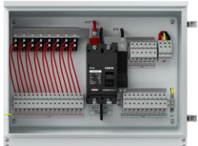
LQT-N/1DC1500VM3
