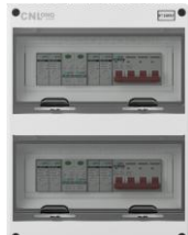
LQX-C4/2DC500VB1
