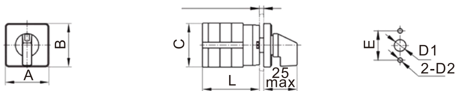
LW26-10/LW26-10G dimensions and mounting dimensions
