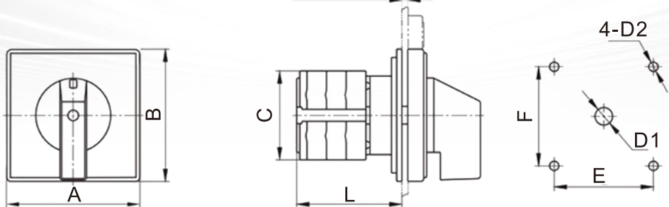
LW26-10/LW26-10G dimensions and mounting dimensions
