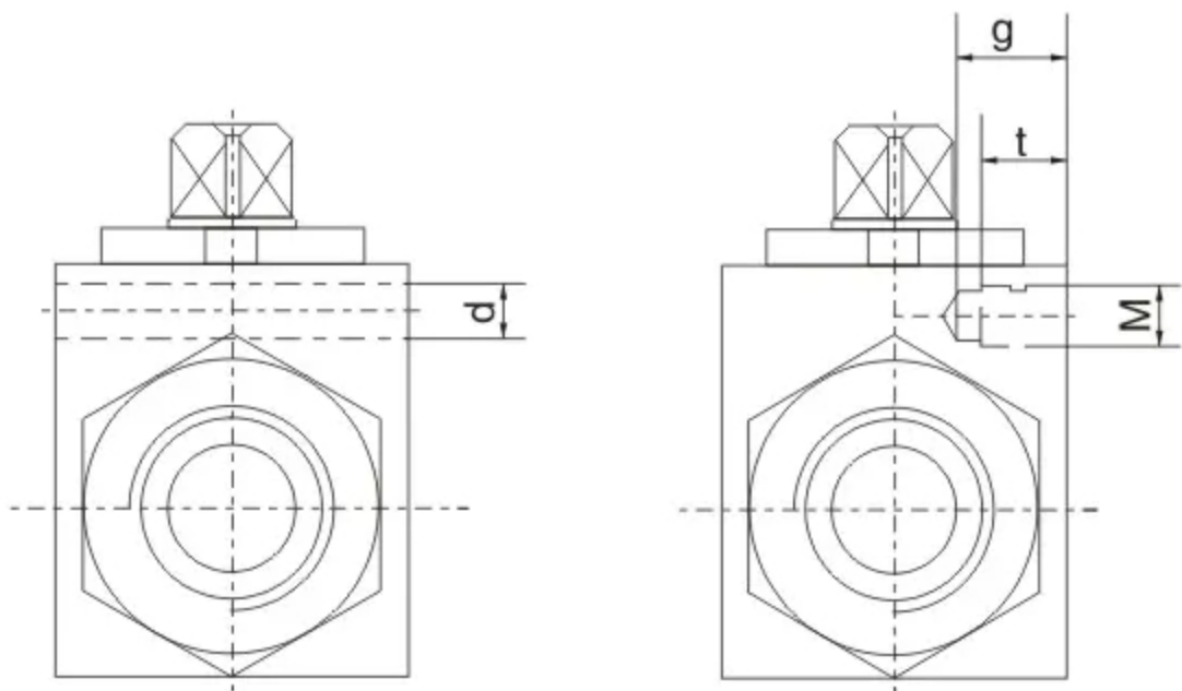
螺纹孔连接尺寸/Thread Holes Dimensions
