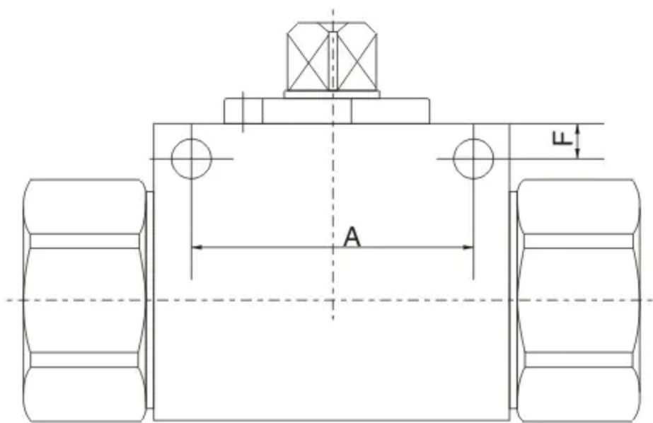
通孔连接尺寸/Full Holes Dimensions
