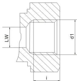
SAE J514
