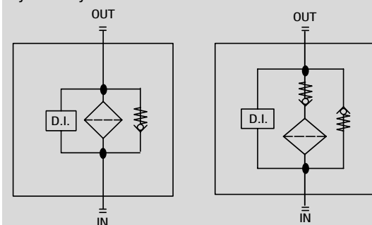
Hydraulic symbols
