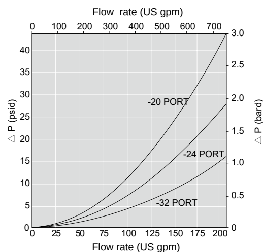
310 Series Filter Elements —bar/1000 l/min (psid/US gpm)
