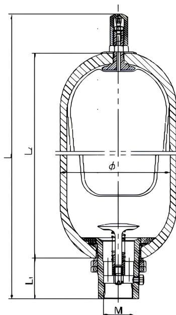
Bottom Repair Construction
