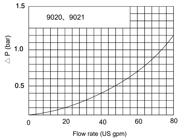
9020 Series Filter Elements —bar/1000 l/min (psid/US gpm)
