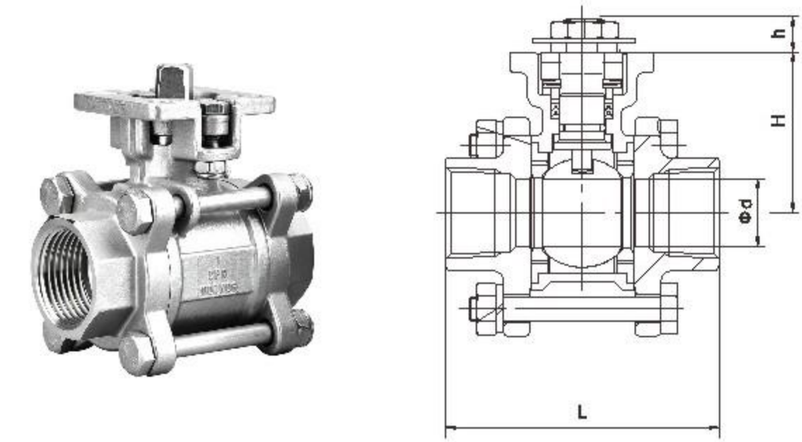
三片式高平台丝扣球阀 3PC High Platform Threaded Ball Valve
