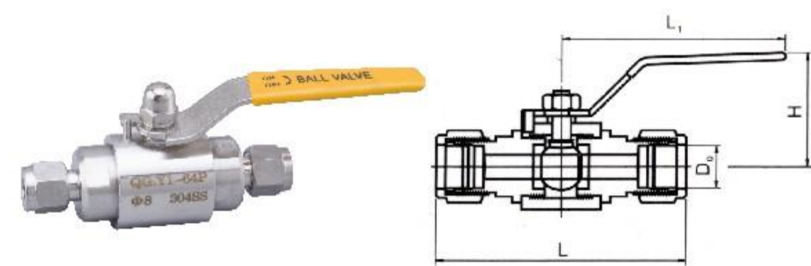
气源球阀 Gas Source Ball Valve
