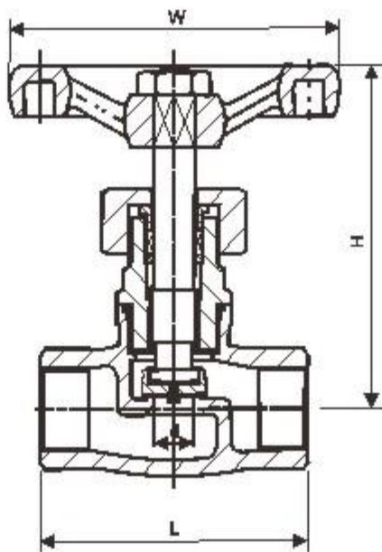
J11W-16P 水暖截止阀 J11W-16P Water Heating Globe Valve
