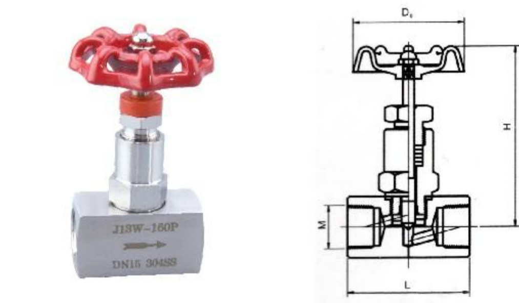
J13W 针型阀 J13W Needle Valve
