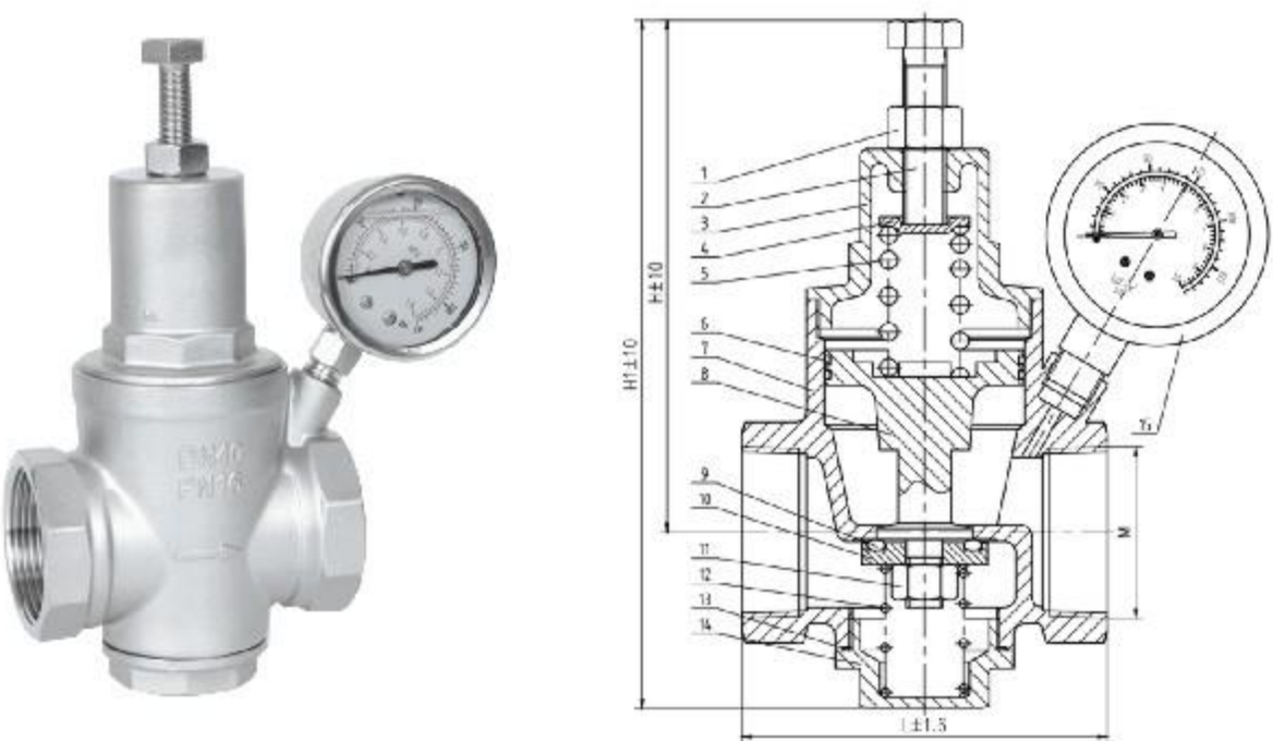
Y12 活塞式减压阀 Y12 Piston Pressure Reducing Valve
